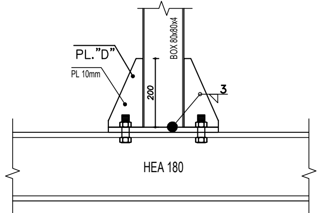
HEA 180 TO BOX 80x3.6 1:10
