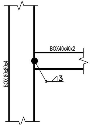
BOX40x40x2 TO BOX 80x80x4 1:10
